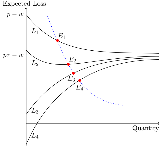
Figure 2: Lottery Equilibria as Inherited Jackpot Rises. This shows lottery equilibria for supply curves with inherited jackpots J_1 < J_2 < J_3 < J_4 from Figure 1.
