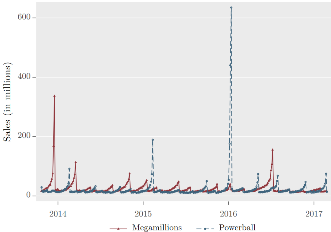
Figure 4: Mega Millions and Powerball sales. This shows the time series of sales (millions of tickets sold nationwide) for Mega Millions and Powerball in our sample.
